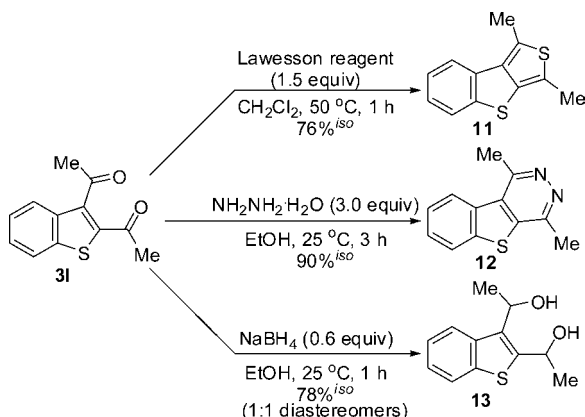
Scheme 4. Synthetic Transformations of 3l
