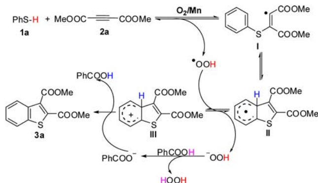
Scheme 5. Tentative Reaction Mechanism
