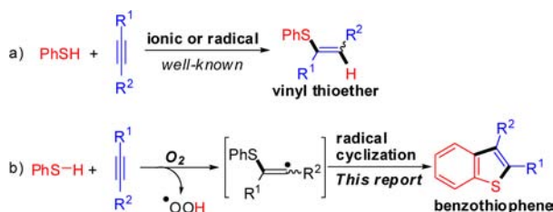
Scheme 1. Reaction Pathways of Thiophenol and Alkynes
