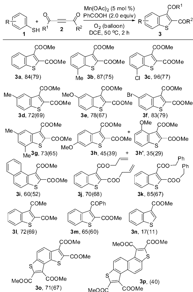
Figure 1. Representative results for the oxidative annulation of thiophenols with alkynes. (a) Conditions: 1 (0.5 mmol), 2 (1.0 mmol), Mn(OAc) 2 (0.025 mmol), PhCOOH (1.0 mmol), DCE (5.0 mL), 50 °C, 2 h, under O 2 (balloon). (b) Reported yields were based on 1 and determined by 1 H NMR using an internal standard; isolated yields are given in parentheses. (c) For synthesis of 3o and 3p , 2a (2.0 mmol) and PhCOOH (2.0 mmol) were used.
